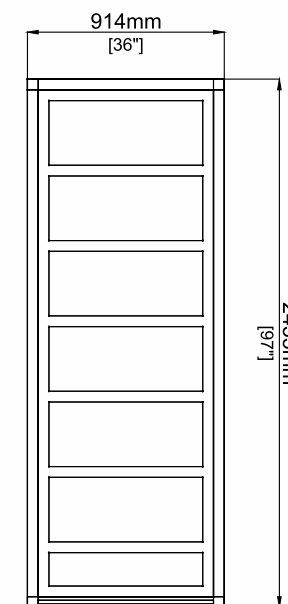
TOP VIEW
